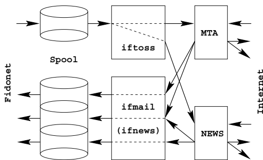
Figure 1: Gateway Structure
