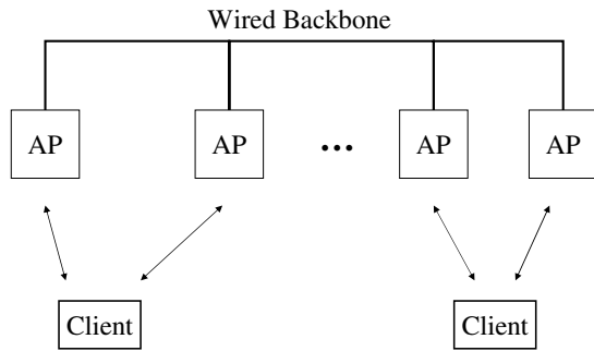
Figure 6: A cellular WLAN model where neighboring APs have overlapping coverage. To achieve the benefits of fine-grained path selection, Divert requires that the client switch between APs quickly and at low cost. Section 3.2 shows how 802.11-like systems can achieve this goal.
