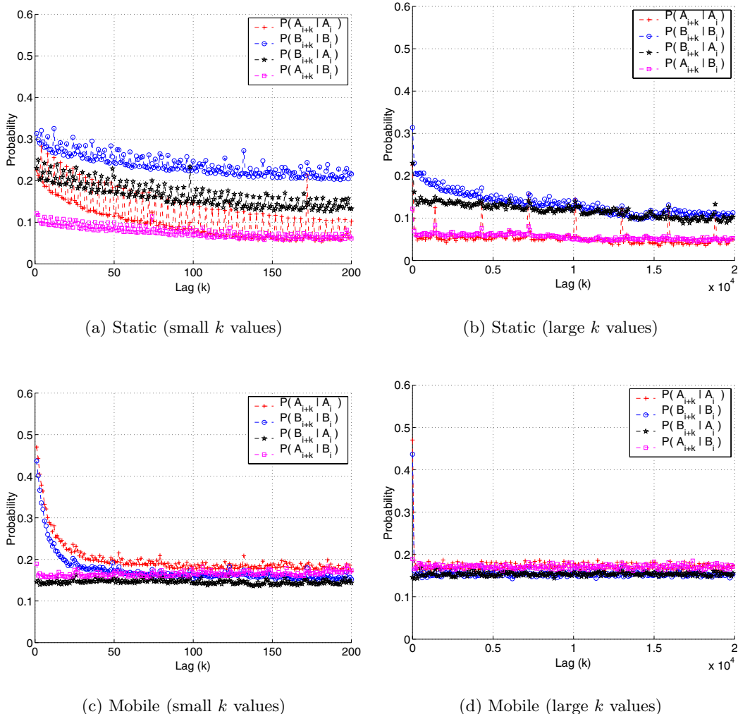
Figure 3: The auto-conditional and cross-conditional loss probabilities of frame losses at different frame lags k for the static (a) and (b) and mobile (c) and (d) experiments.
