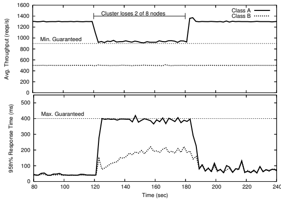
Figure 11: Quorum’s reaction to a failure of 2 nodes.
