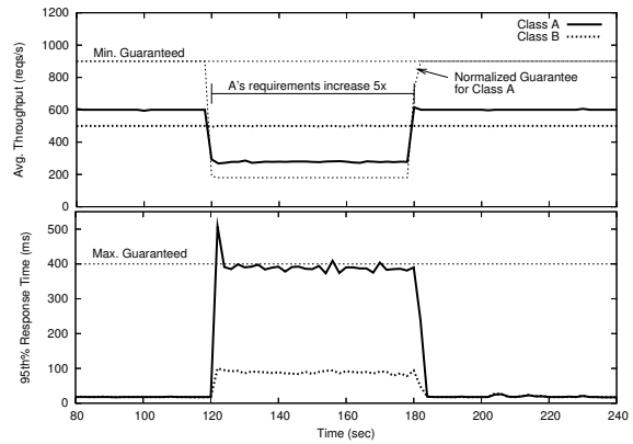
Figure 10: Behavior of Quorum when requests of class A suddenly require five times more resources for their computation.
