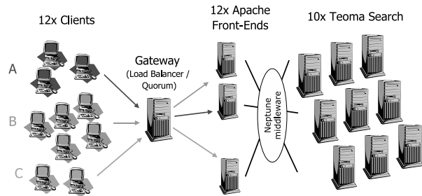
Figure 7: Experimental test-bed used for our benchmark using Teoma’s search service.
