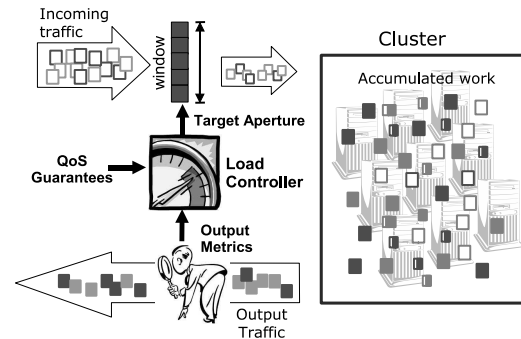
Figure 4: Structure of Load Control module.
