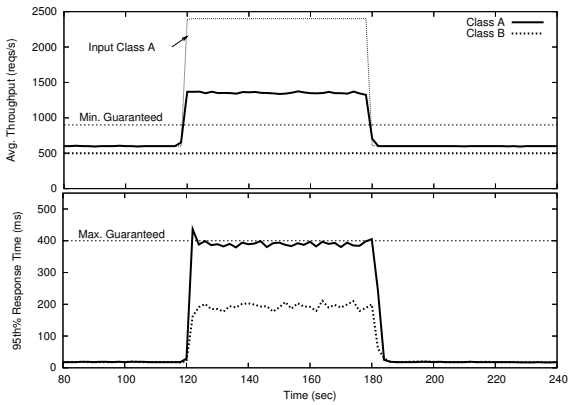
Figure 9: Quorum’s reaction to extreme fluctuation of incoming traffic.
