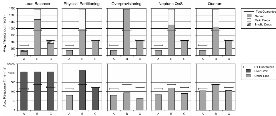
Figure 8: Experimental comparison of current approaches and Quorum, using Teoma's search engine.
