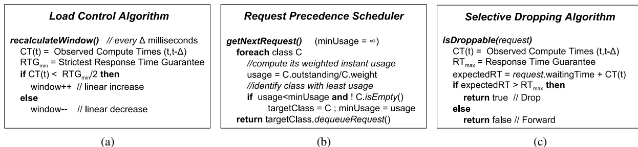
Figure 3: Simplified pseudo-code for the algorithms of the three main modules of Quorum.
