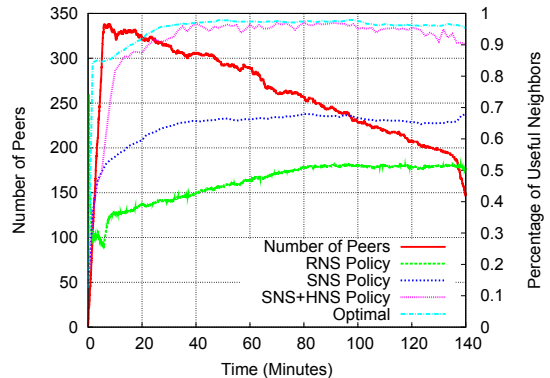
Figure 2: Comparison of Peer Selection Algorithms at the Tracker.
