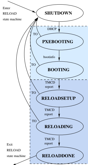
Figure 1: The Emulab node-imaging state machine.
