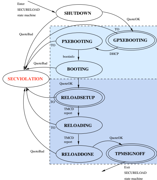
Figure 2: The Emulab TDLS state machine.
