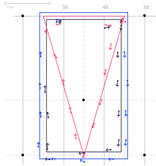
Figure 10: Simultaneous tracking of multiple nodes: a person holds two notes in two hands, approximately 1.5 m apart and walks on the rectangular track, second person holds a single note and walks on the triangular track.
