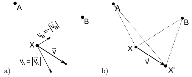
Figure 3: Doppler effect in radio interferometric ranging.
