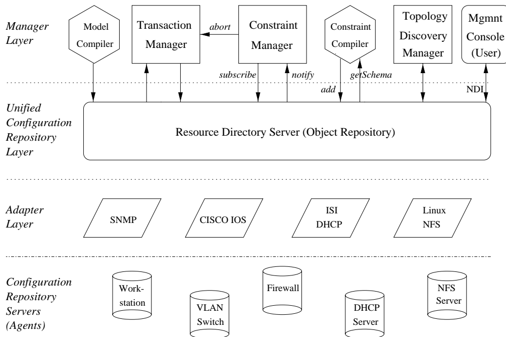
Figure 1: NESTOR Architecture.
