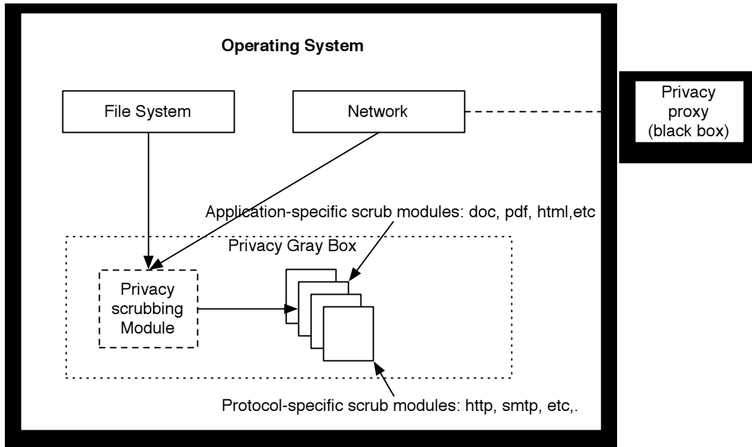
Figure 1: Architectural overview: A privacy-servicing module lives inside the operating system. File and network requests as well as other relevant system calls are redirected to this module where scrubbing happens. The privacy module can be extended with application- or protocol-aware modules. For a purely network-oriented architecture, the privacy module can be a proxy “black box” that scrubs traffic on the fly.
