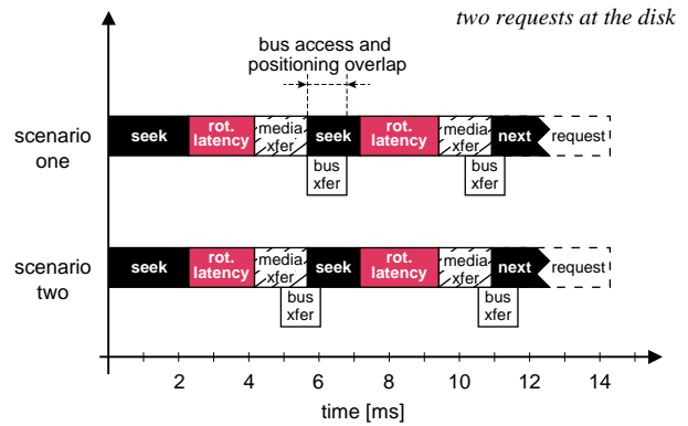
Figure 4: Limited command queuing. This figure repeats the two scenarios from Figure 2 but with two requests outstanding at the drive. That is, the scheduler keeps two requests at the disk — in this example, request A is being serviced while request B is queued. The drive completely overlaps the bus transfer of request A with the seek of request B , eliminating head idle time. Also, notice that the rotational latency is the same in both scenarios, making predictions easier for foreground and freeblock schedulers.
