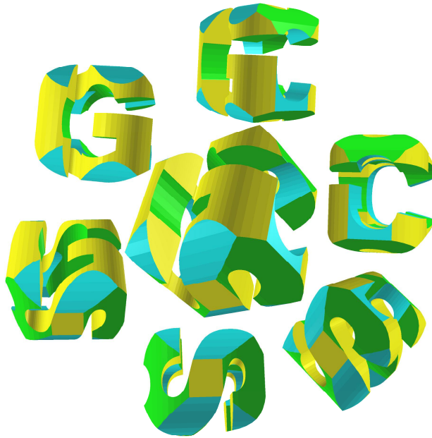
Figure 7. How does a 3D object look like that exactly fits through all letter-shaped holes? CSG gives the answer: Just intersect the extruded 3D-models of each letter. The resulting shape is shown below from different positions.
