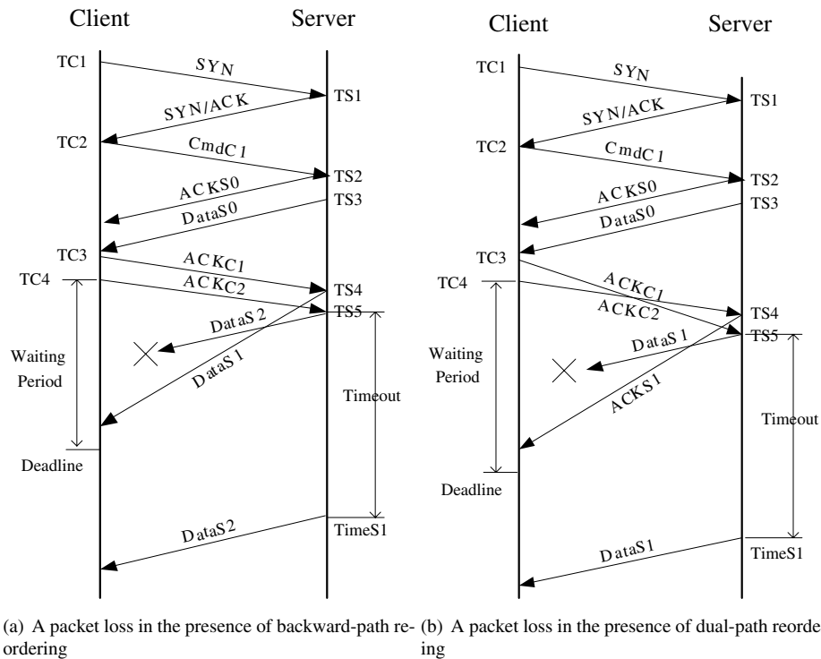
Figure 4: Handling packet losses in the ACM method.
