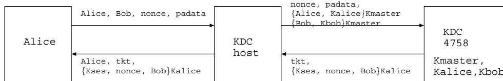
Figure 2: AS_REQ processing in Kerberos V5 with the 4758
