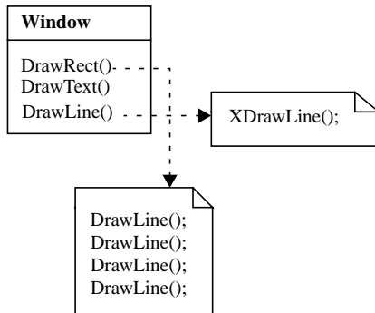
Figure 3.9: Design for a single window system
