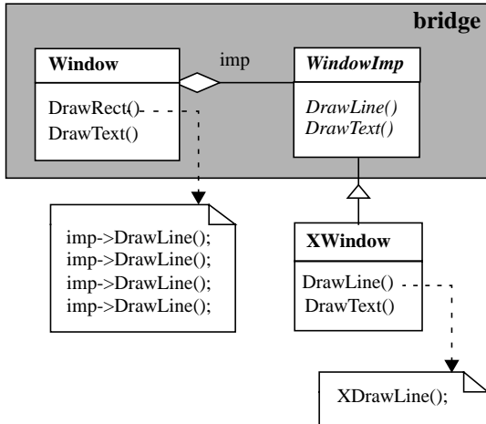
Figure 3.8: Bridge design pattern example
