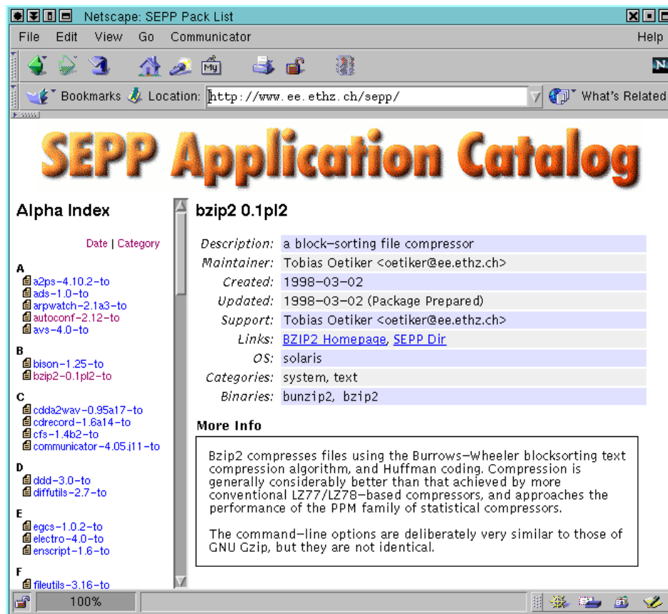
Figure 2: SEPP generated Documentation Web Site.
