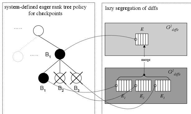
Figure 7: Lazy segregation
