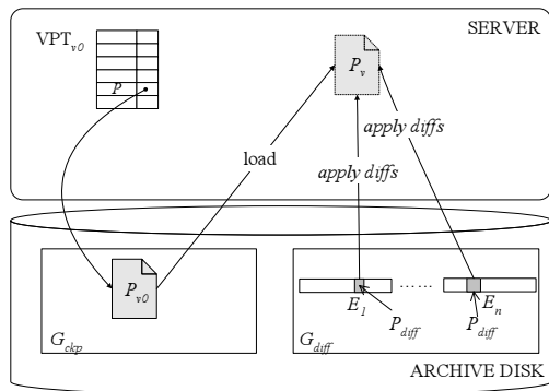
Figure 6: BITE: diff-based representation
