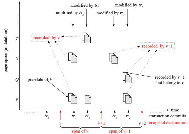
Figure 2: Split copy-on-write
