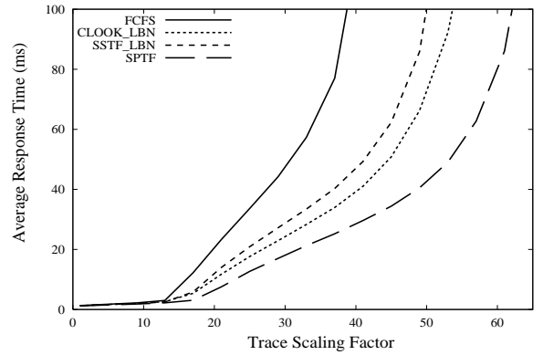
(b) TPC-C average response times
