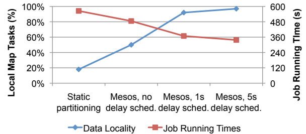
Figure 8: Data locality and average job durations for 16 Hadoop instances running on a 93-node cluster using static partitioning, Mesos, or Mesos with delay scheduling.
