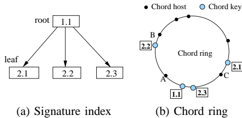
Fig. 3. Storing the signature index nodes on a Chord ring
