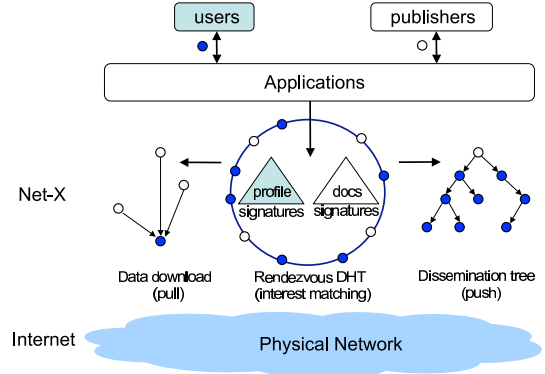
Fig. 2. Overview of Net-\mathcal{X}
