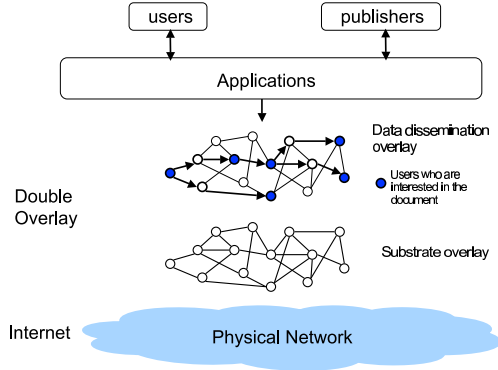
Fig. 1. Double-overlay adopted in previous work
