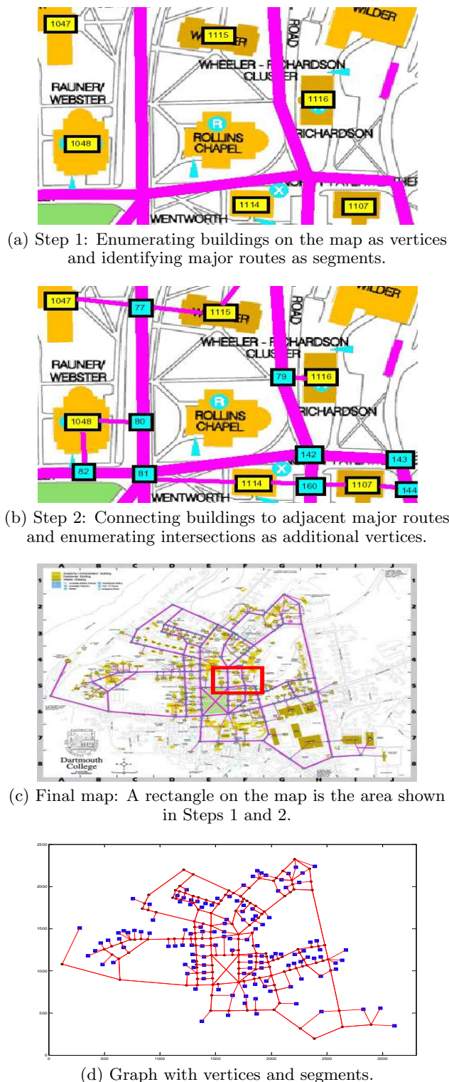
Figure 5: Converting a map to a graph
