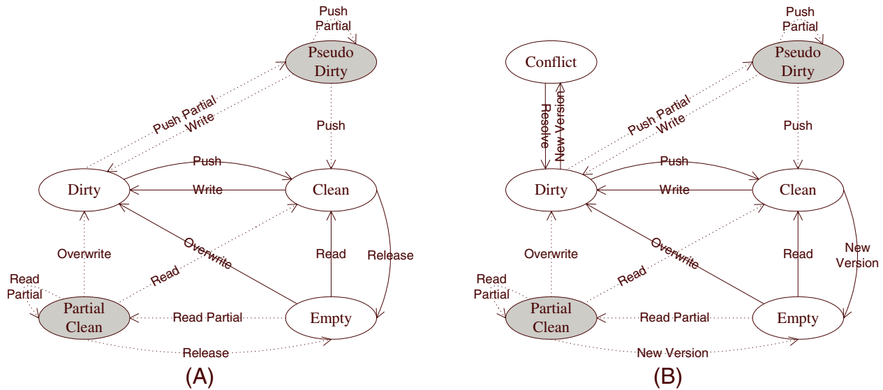
Figure 4: State transition diagrams for individual components of client replicas that support partial document editing and progressive update propagation based on pessimistic (A) and optimistic (B) replication models.
