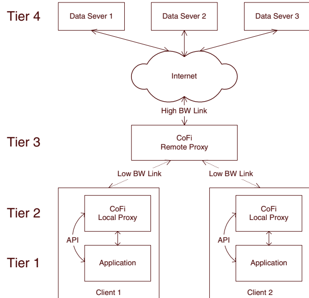
Figure 5: CoFi architecture.
