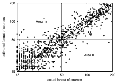
Figure 9: Actual vs. estimated fan-out of sources for trace IPKS+ with flow sampling rate 1/4. The aforementioned second definition of source and destination labels is used here. Note that both x-axis and y-axis are on logscale.
