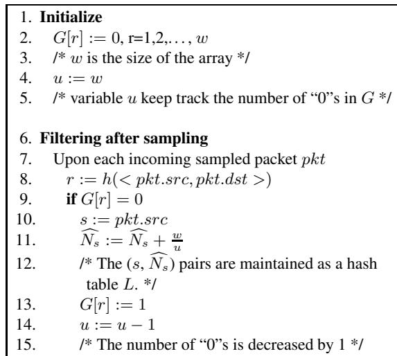
Figure 2: Algorithm of updating data streaming module.
