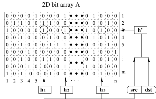
Figure 4: An instance of online streaming module
