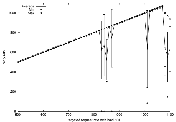
FIGURE 9. httpd modified to use /dev/poll , with 501 extra inactive connections. Despite some response rate anomalies, the modified server manages a high inactive connection load with ease. Performance begins to break down at extreme high request rates.
