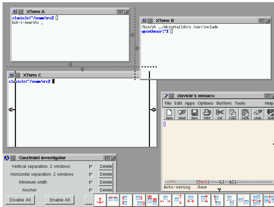
Figure 3: Visual representation of constraints. XTerm A is constrained to be to the left of XTerm B, and above XTerm C. Additionally, XTerm C is required to have a minimum width, and the XEmacs window's southeast corner is anchored at its current location. The constraint investigator that allows users to manage the constraints instances appears in the bottom left of the screen shot.
