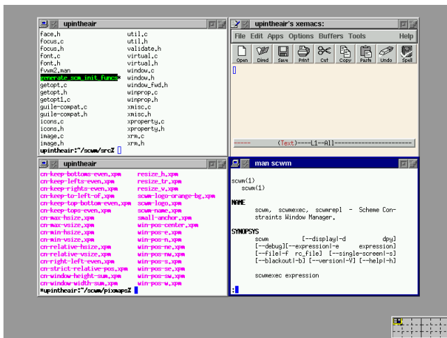
Figure 4: Four windows tiled together. Unlike tiled-only window managers, SCWM permits users to tile a subset of their windows; other windows could overlap arbitrarily.
