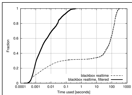
Figure 11: Overall Processing Time, Blackbox testing BGP updates and Path cost changes combined: All path cost changes (unfiltered) and filtered path cost changes
