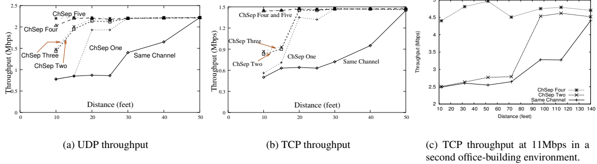
Figure 3: TCP/UDP throughputs versus spatial separation ( ChSep ).
