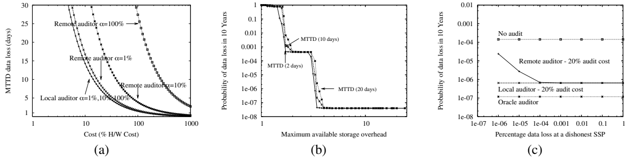
Fig. 5: (a) Time to detect SSP data loss via audit with varying amounts of resources dedicated to audit overhead assuming honest SSPs. (b) Durability with varying MTTD. (c) Impact on overall durability with a dishonest SSP. The audit cost model for hardware, storage, and network bandwidth are described in [45]
