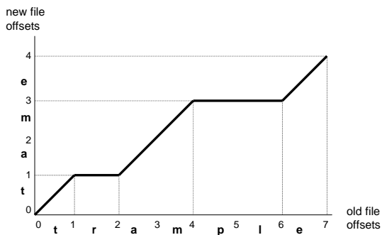
Figure 6: Coordinate map translating offsets between two versions of a file. The old version is the word trample . Two regions are deleted to get the new version, tame .
