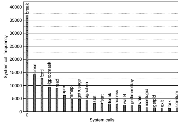
Figure 10: Histogram of system call frequency for compilation benchmark. The performance impact of application confinement depends mostly on the number of system calls that require a policy decision by the user space daemon. The histogram shows that the most frequent system calls can be handled by the in-kernel policy.
