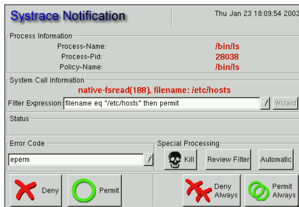
Figure 2: A graphical notification assists the user when a policy decision is required. A user may decide to allow or deny the current system call or to refine the policy.
