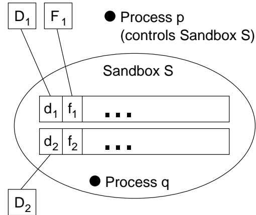
Figure 1: Blocking mechanism
