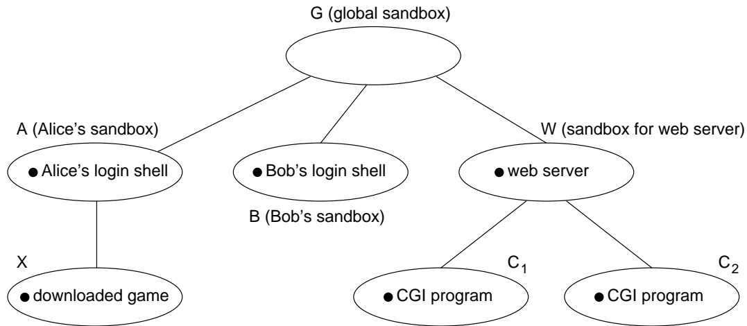
Figure 2: Nested sandboxes
