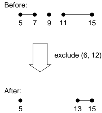
Figure 4: Exclude operation
