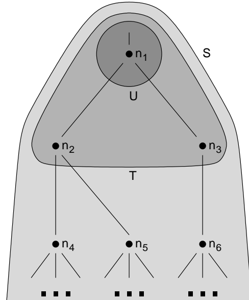
Figure 6: Directory subtree
