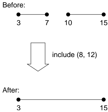
Figure 3: Include operation
