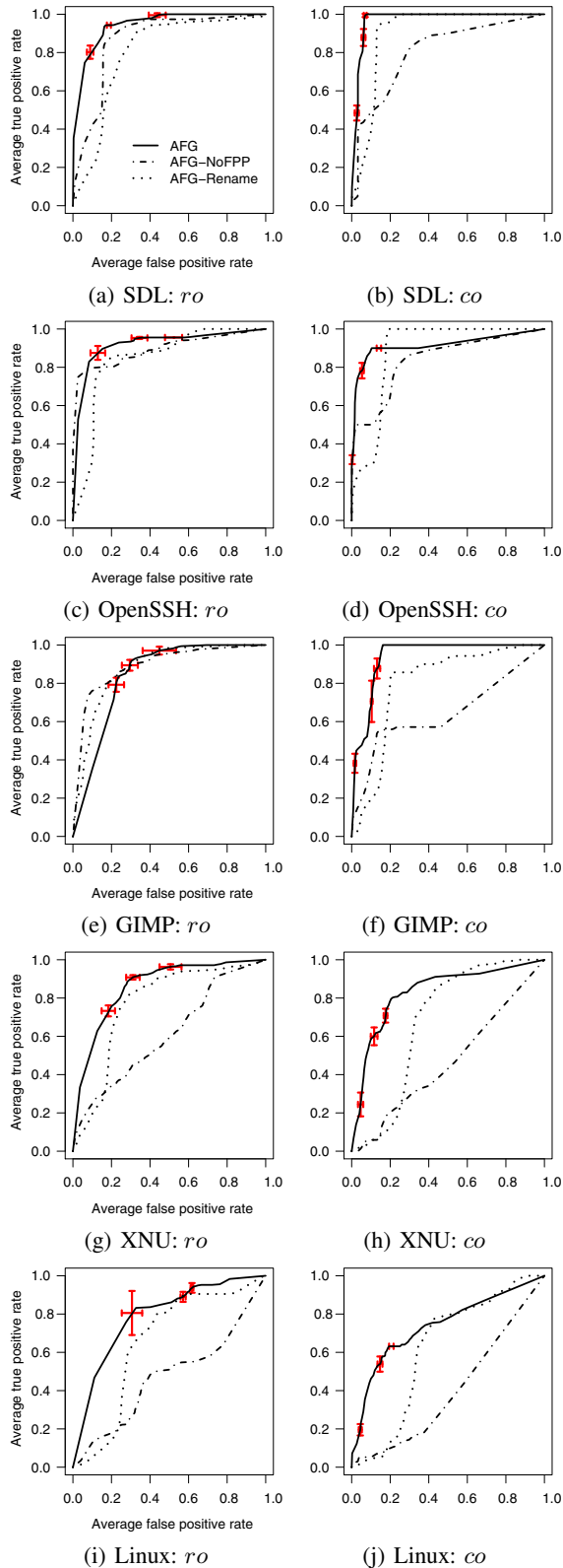
Figure 7: ROC curves depicting accuracy of inferred annotations. Results are averaged over 10 runs where we add Gaussian noise to AFG parameters. Error bars (shown at the classification probability thresholds of 0.95, 0.7, and 0.4) depict standard deviations.
