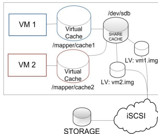
Figure 1. DM-cache share cache feature
